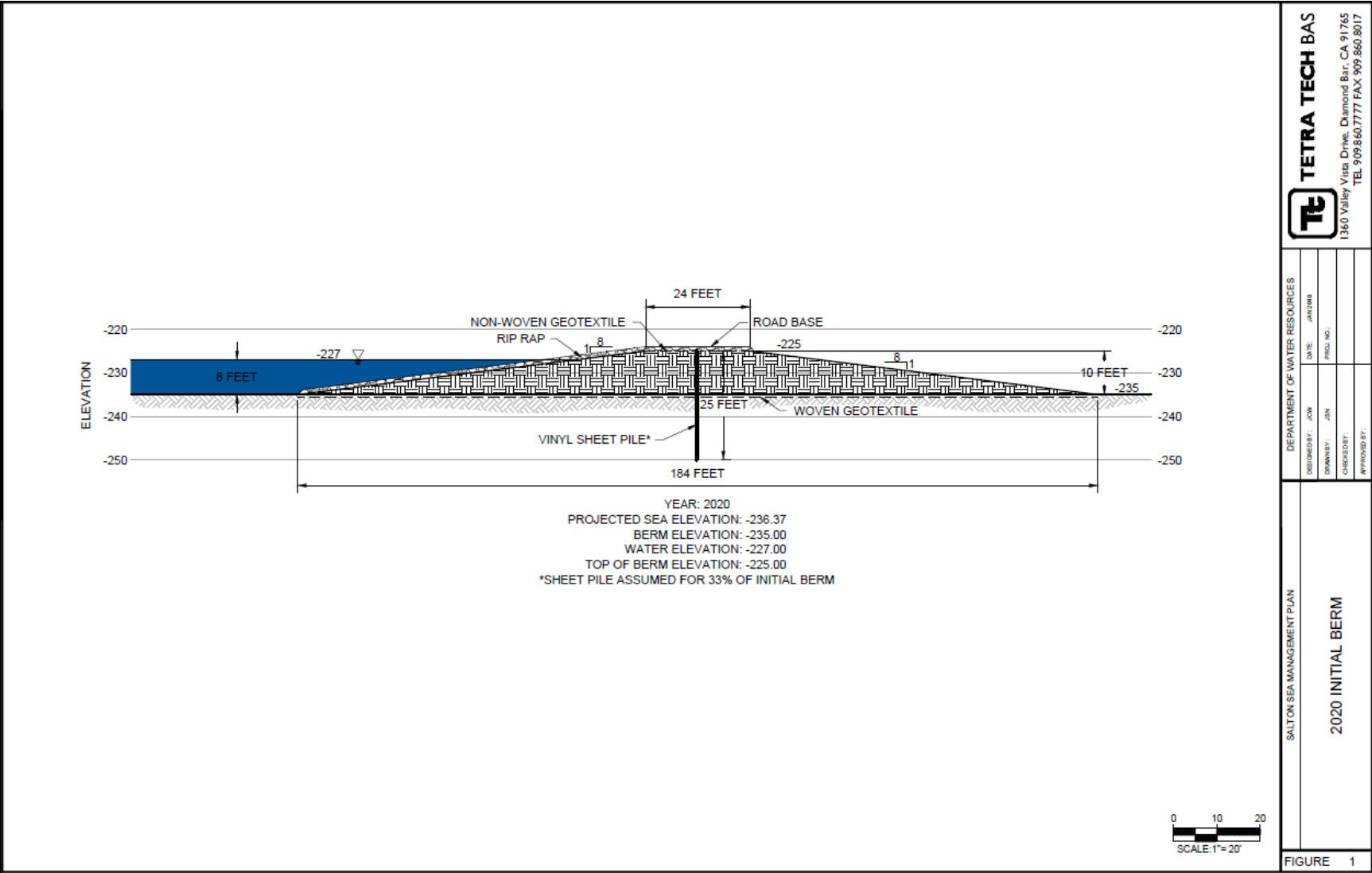
Figure A-5 2020 Initial Berm Cross Section
