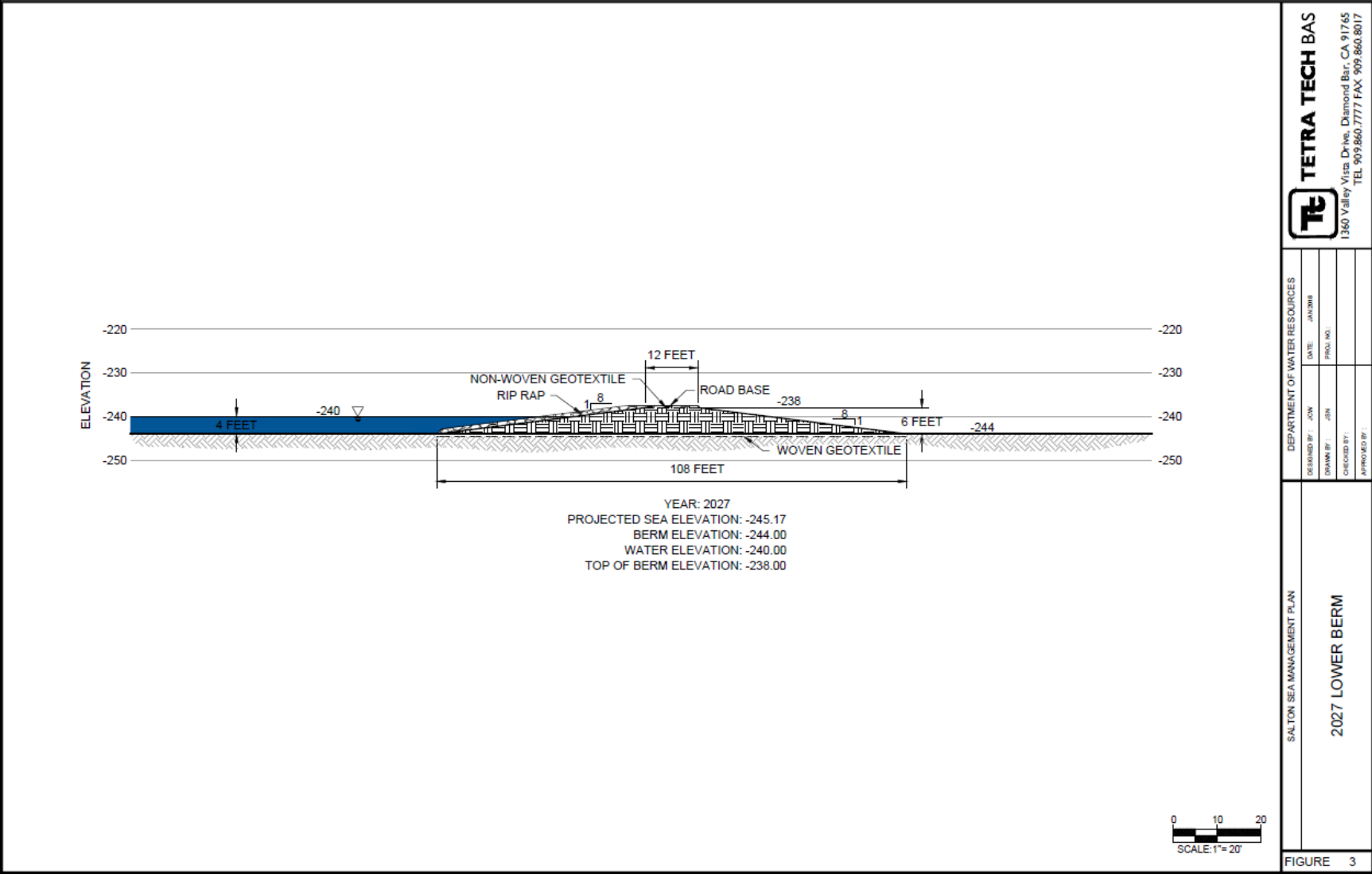
Figure A-7 2027 Lower Berm Cross Section
