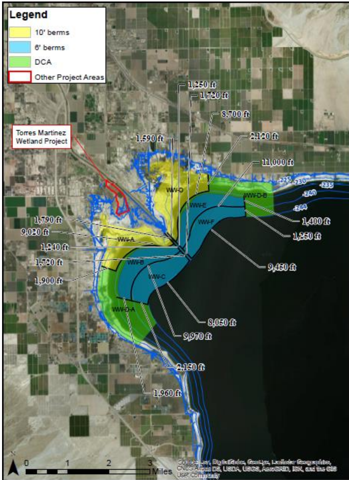
Figure A-4 Berm Configuration for Whitewater River
