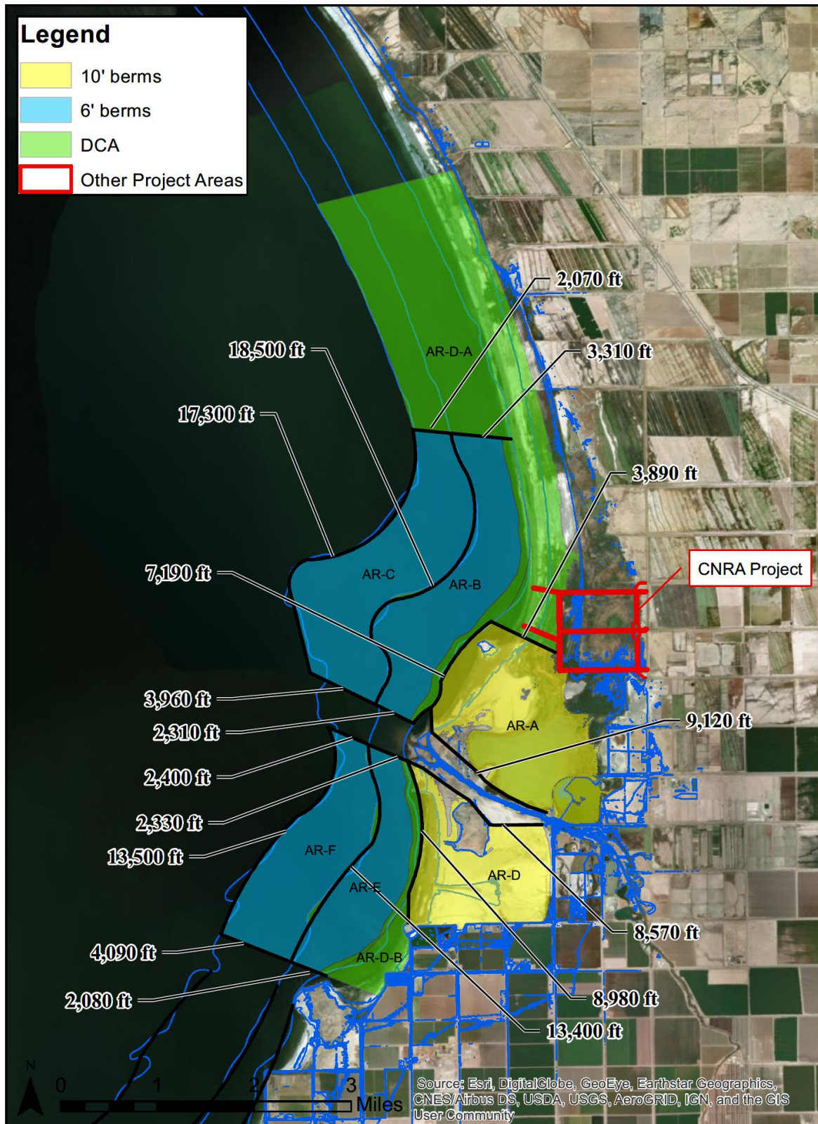
Figure A-3 Berm Configuration for Alamo River
