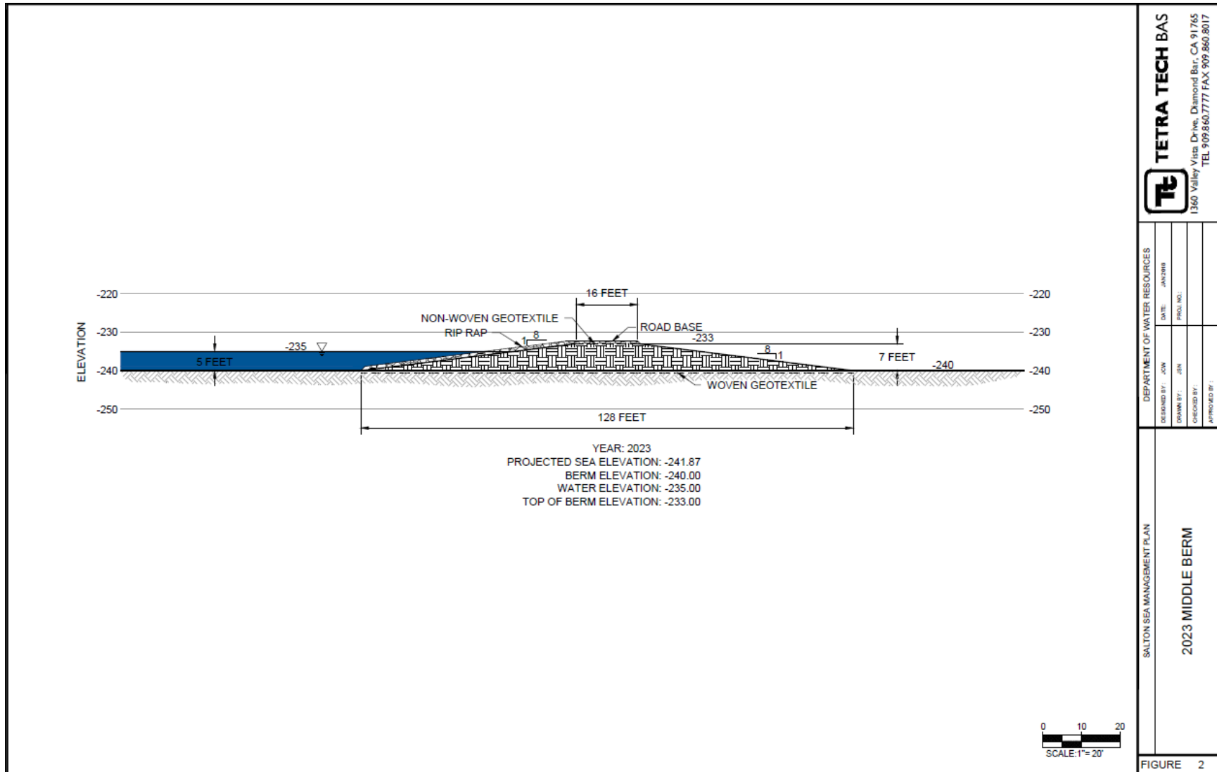
Figure A-6 2023 Middle Berm Cross Section
