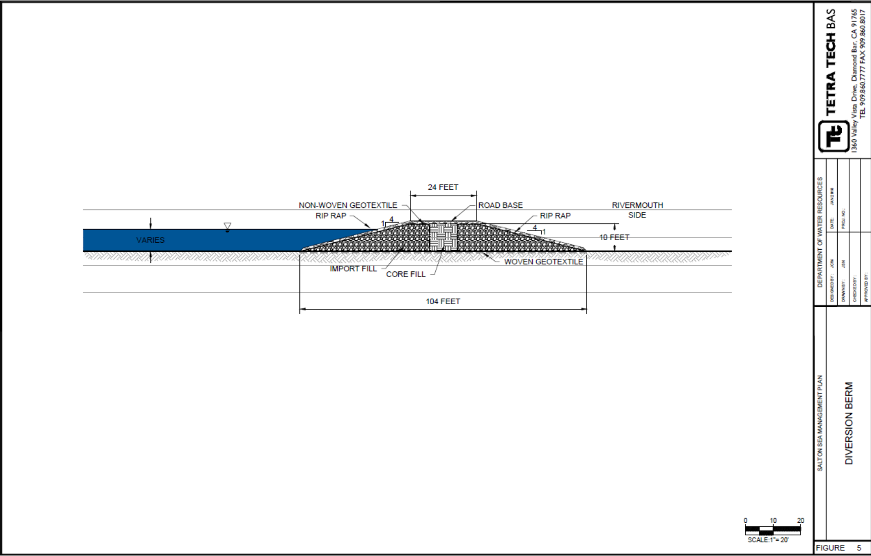
Figure A-9 Diversion Berm Cross Section
