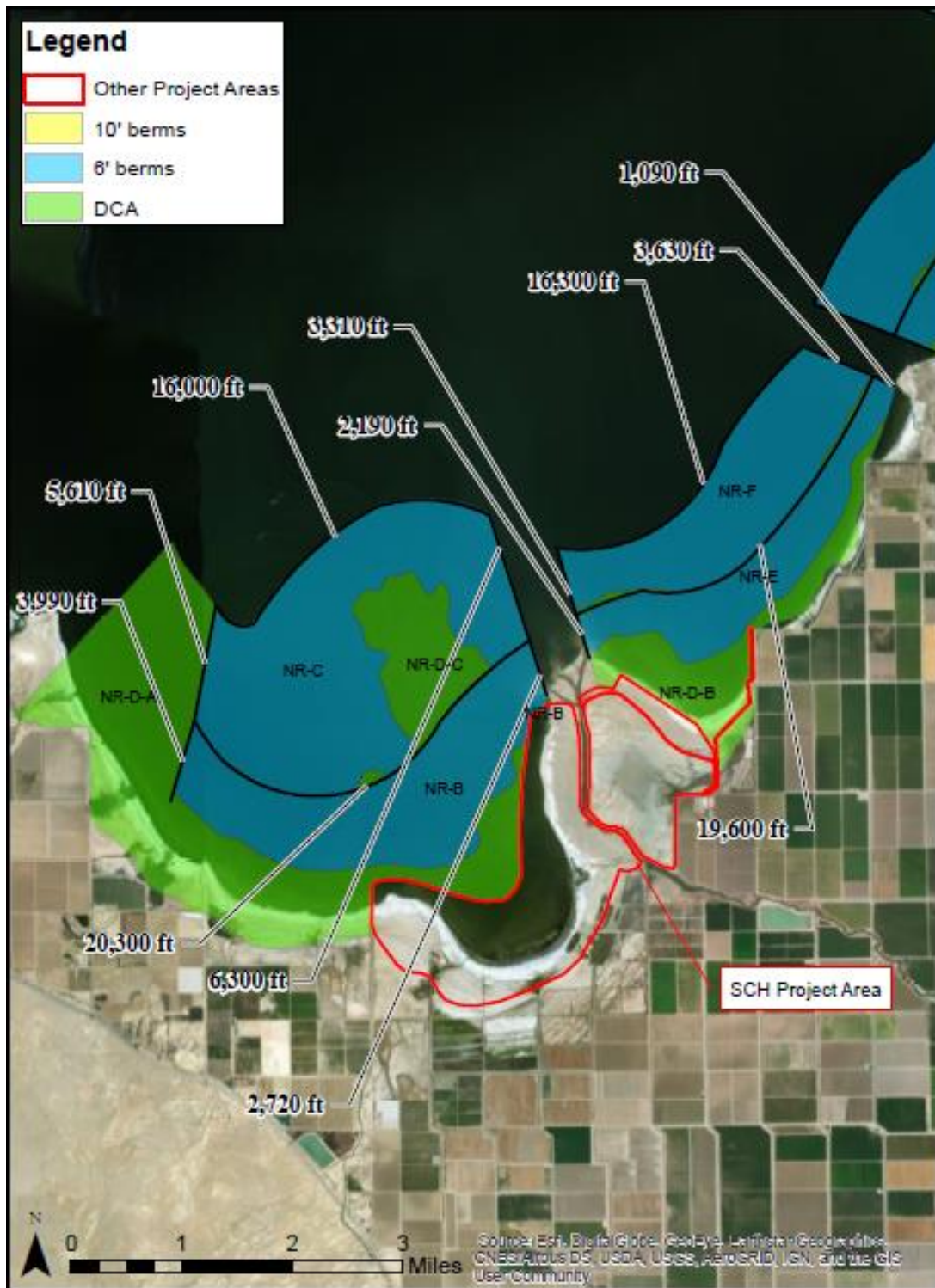
Figure A-2 Berm Configuration
