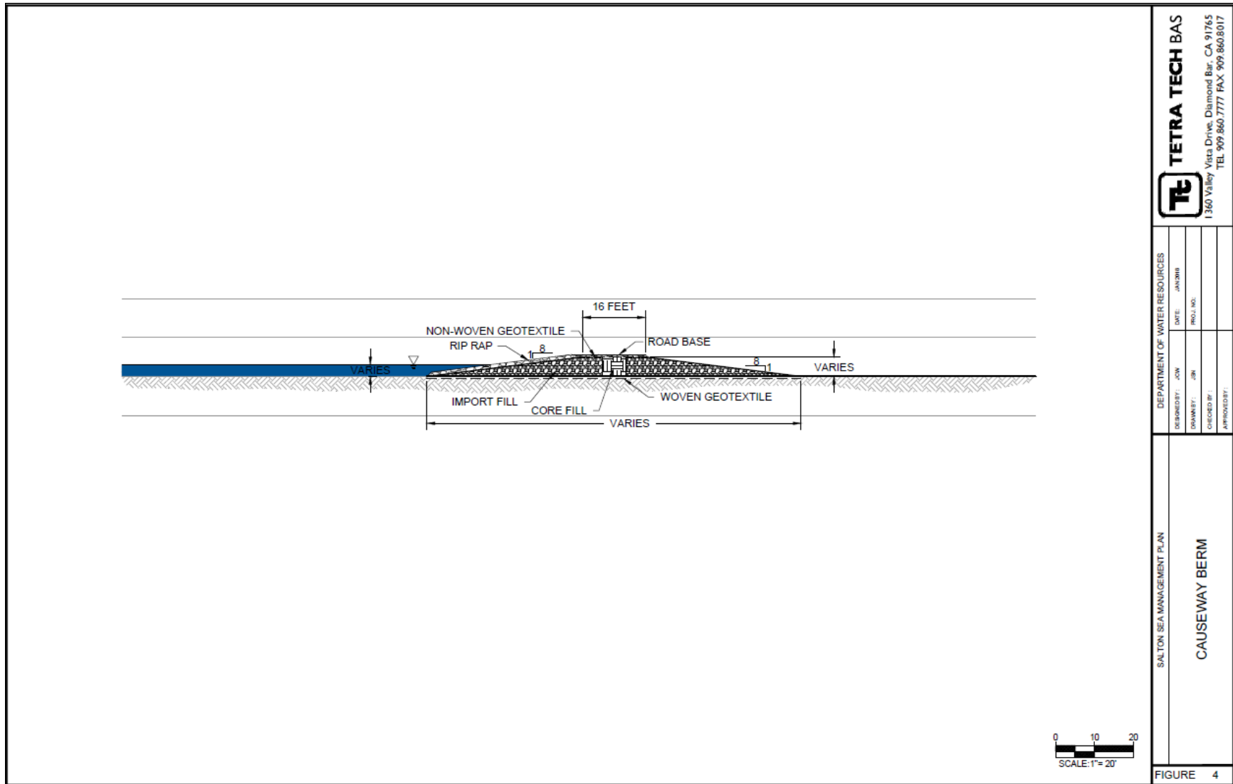
Figure A-8 Causeway Berm Cross Section
